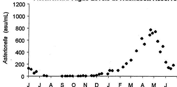
Asterionella Algae Levels at Wachusett Reservoir
