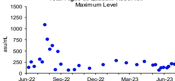
Total Algae at Quabbin Reservoir Maximum Level
