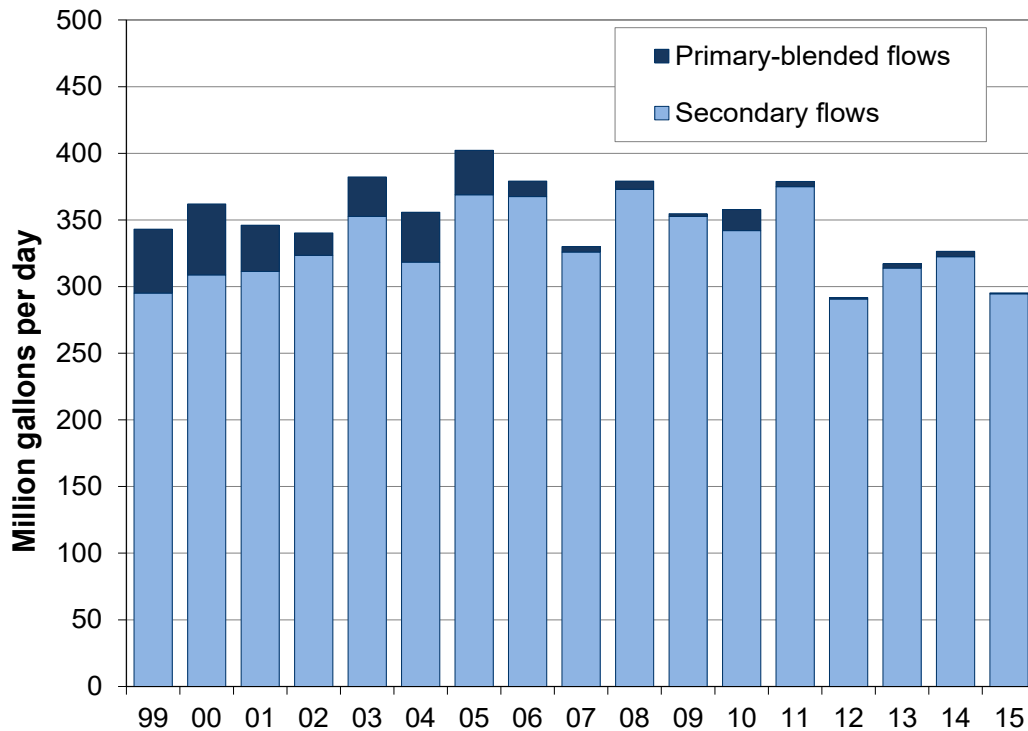
Figure 2-2. Annual primary-blended and full secondary effluent flows, 1999–2015. During large storms, flow exceeding the secondary capacity of the plant is diverted around the secondary process to prevent washing out the essential microbes that carry out secondary treatment. These primary-treated flows are then combined (“blended”) with full secondary flows before disinfection and discharge. All 2015 discharges met permit limits.
