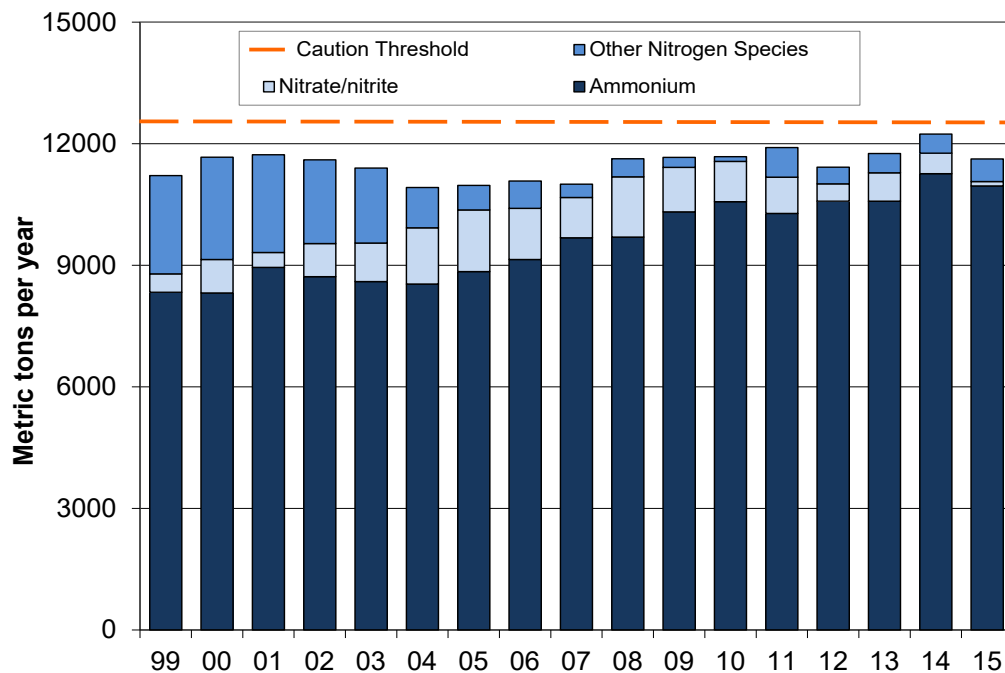
Figure 2-5. Annual nitrogen discharges, 1999–2015. Most of the nitrogen in the effluent is in the form of ammonium.
