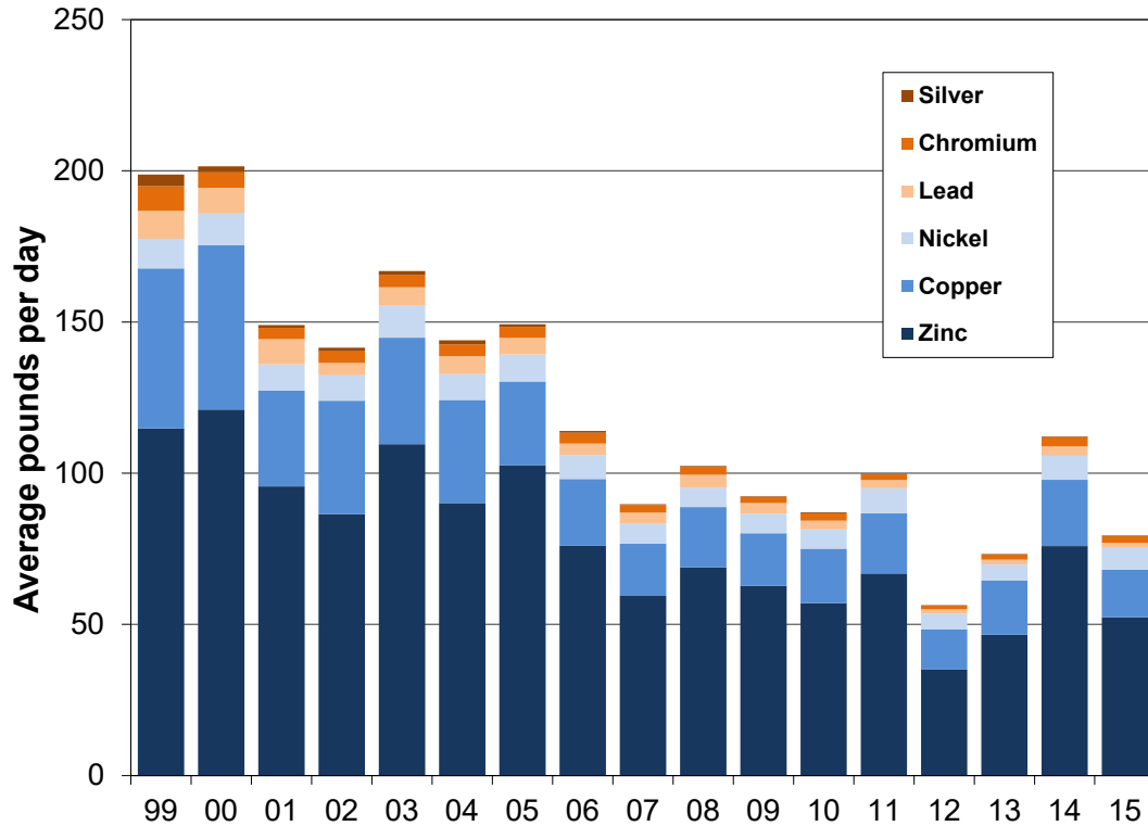
Figure 2-6. Annual metals discharges, 1999–2015.
