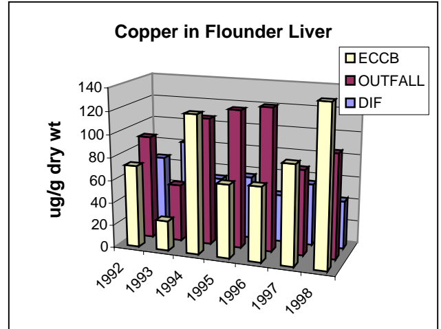
Figure 3-7c. Total Copper in Flounder Liver at DIF, Outfall and ECCB from 1992-1998.
