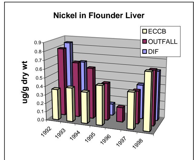
Figure 3-7d. Total Nickel in Flounder Liver at DIF, Outfall and ECCB from 1992-1998.
