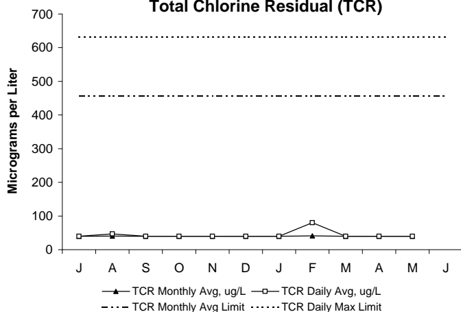
Total Chlorine Residual (TCR)
