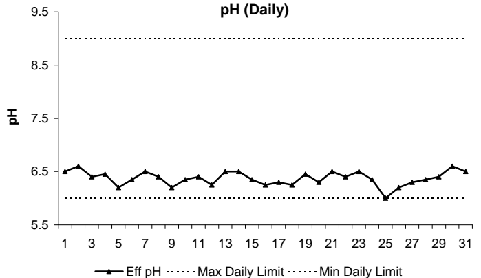
pH (Daily)
