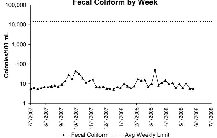
Fecal Coliform by Week
