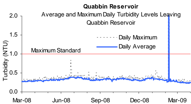
In February, there was a spike in turbidity at Quabbin, but it did not disrupt disinfection effectiveness and was not a violation.
