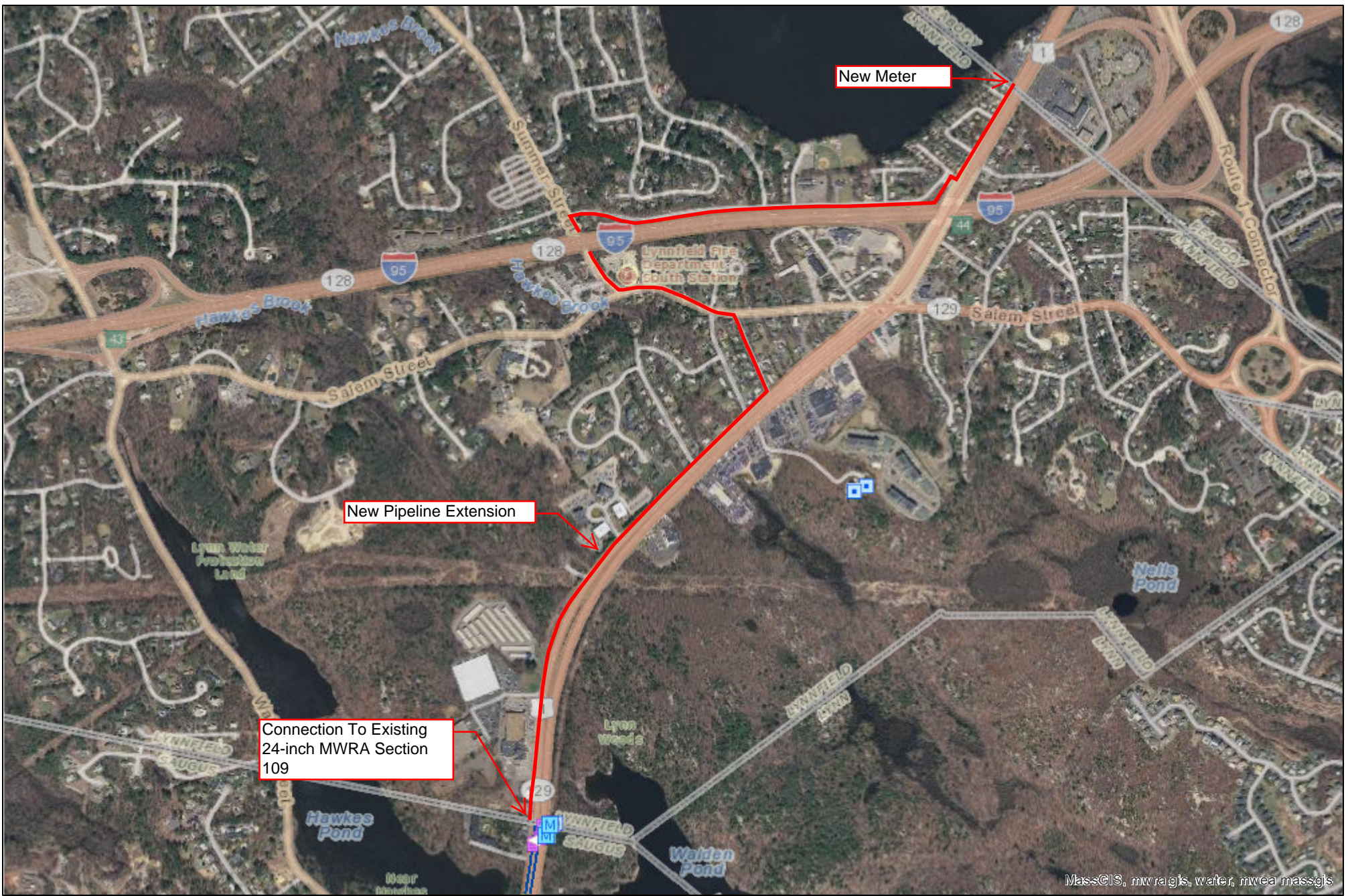
Figure 1 - Contract 6895 - Section 109 Extension, Conceptual Alignment
