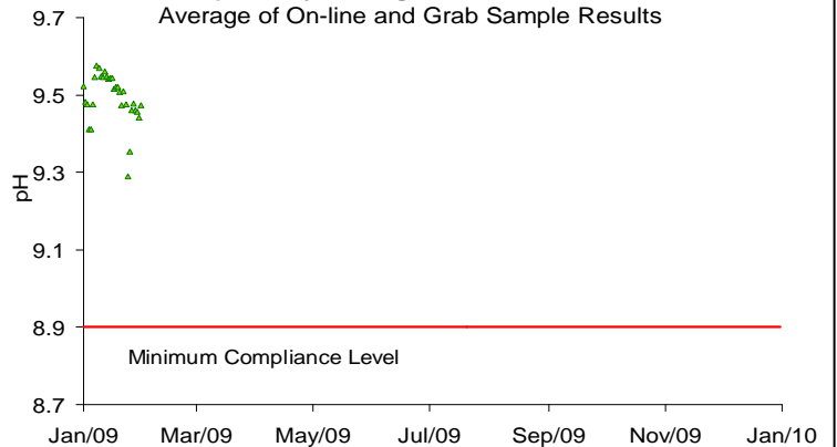
pH Daily Average at CWTP Fin A Average of On-line and Grab Sample Results
