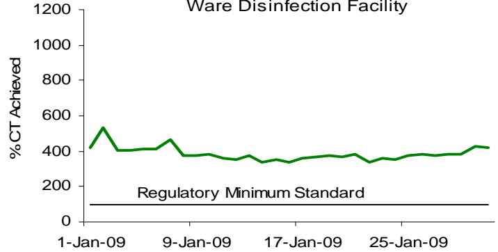
Giardia CT Percent Achievement Ware Disinfection Facility
