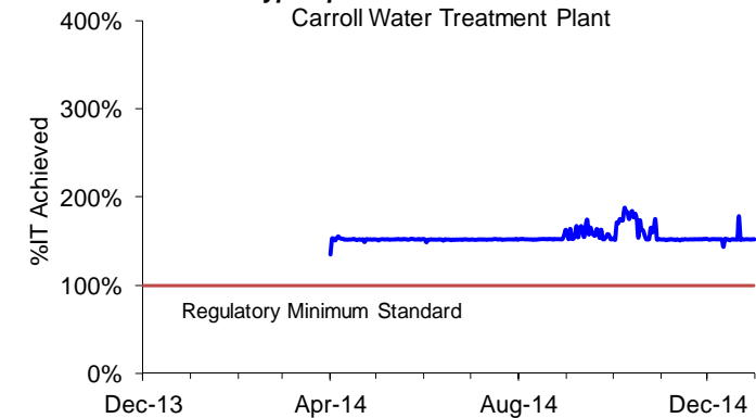
Cryptosporidium IT Percent Achieved Carroll Water Treatment Plant
