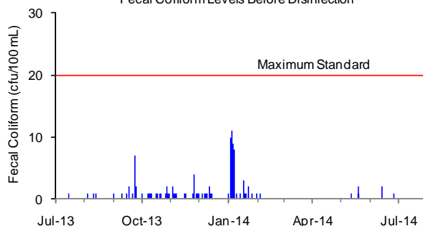
Quabbin Reservoir Fecal Coliform Levels Before Disinfection
