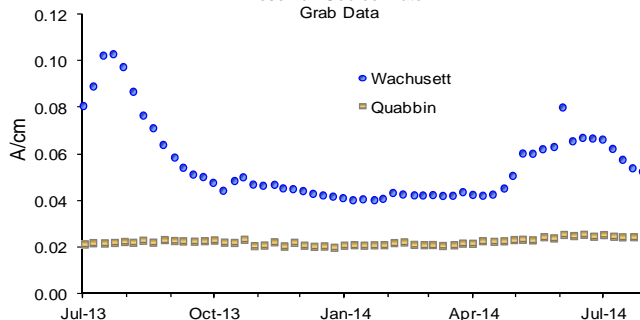
UV 254 Reservoir Source Water Grab Data
