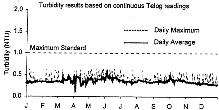
Shaft 4, Wachusett Reservoir
