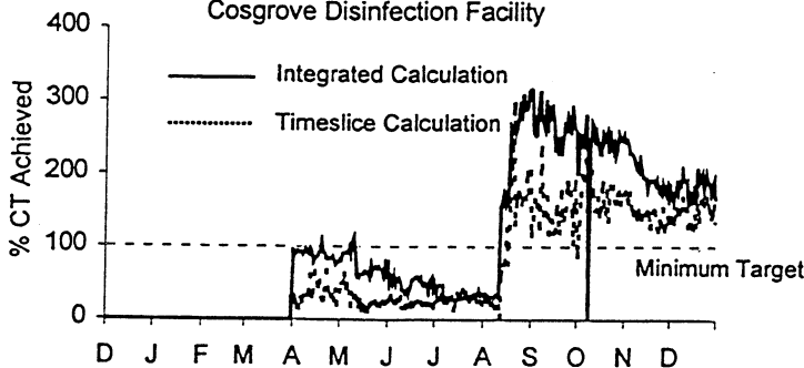
Giardia CT Percent Achievement Cosgrove Disinfection Facility
