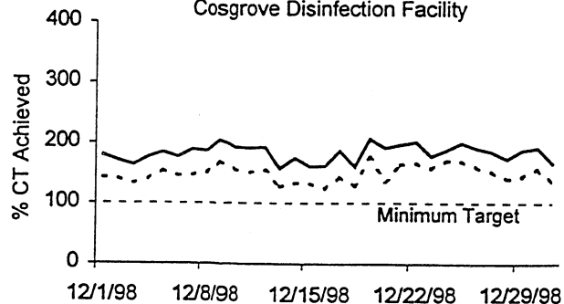
Giardia CT Percent Achievement Cosgrove Disinfection Facility
